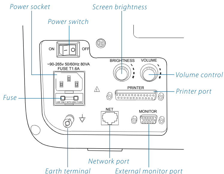
L403 - Back view
